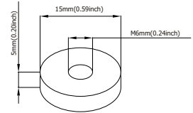
Terminal Dimensions
