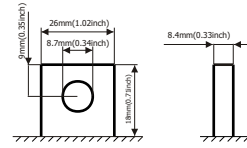
Terminal Dimensions
